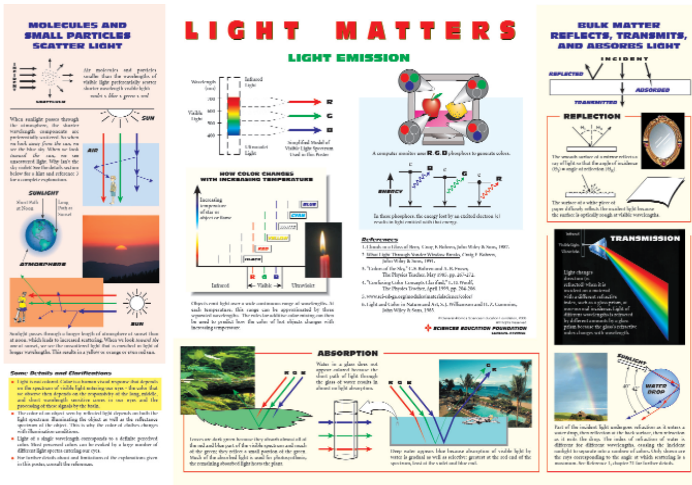
Figure 2. Light Matters Poster—This color poster describes the interaction of light with matter using pictures, diagrams and a written description. The poster is divided into three sections: light scattering, light emission, and the reflection, transmission, and absorption of light by matter.
