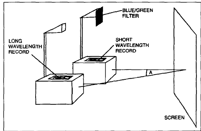
FIGURE 1. SET-UP FOR VIEWING COLOR IMAGE USING TWO BLACK AND WHITE TRANSPARENCIES AND A SINGLE COLOR FILTER.
